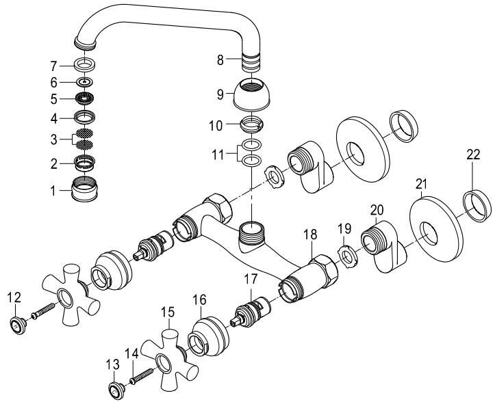
Cold Handle: KSH3221PXC
